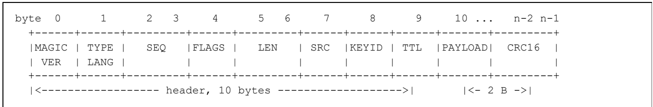
Figure 2.2: Frame format.
